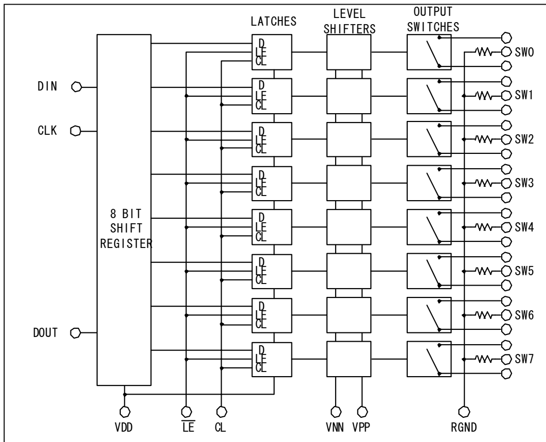
Fig.1 Block diagram
