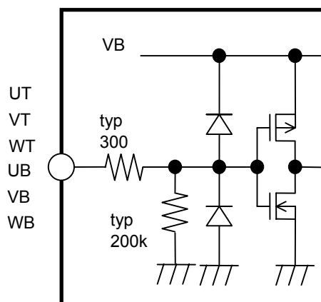
Figure 2. Equivalent circuit around UT, VT, WT, UB, VB, WB
