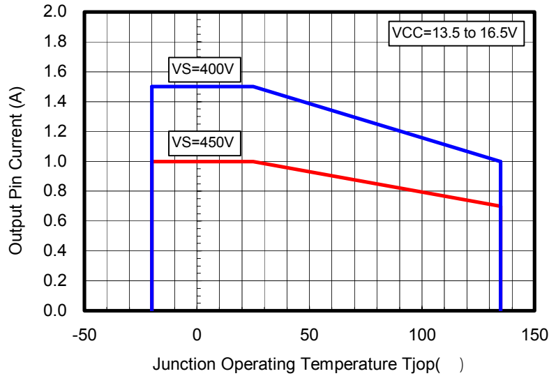
Figure 7. Current Derating for Junction Operating Temperature
