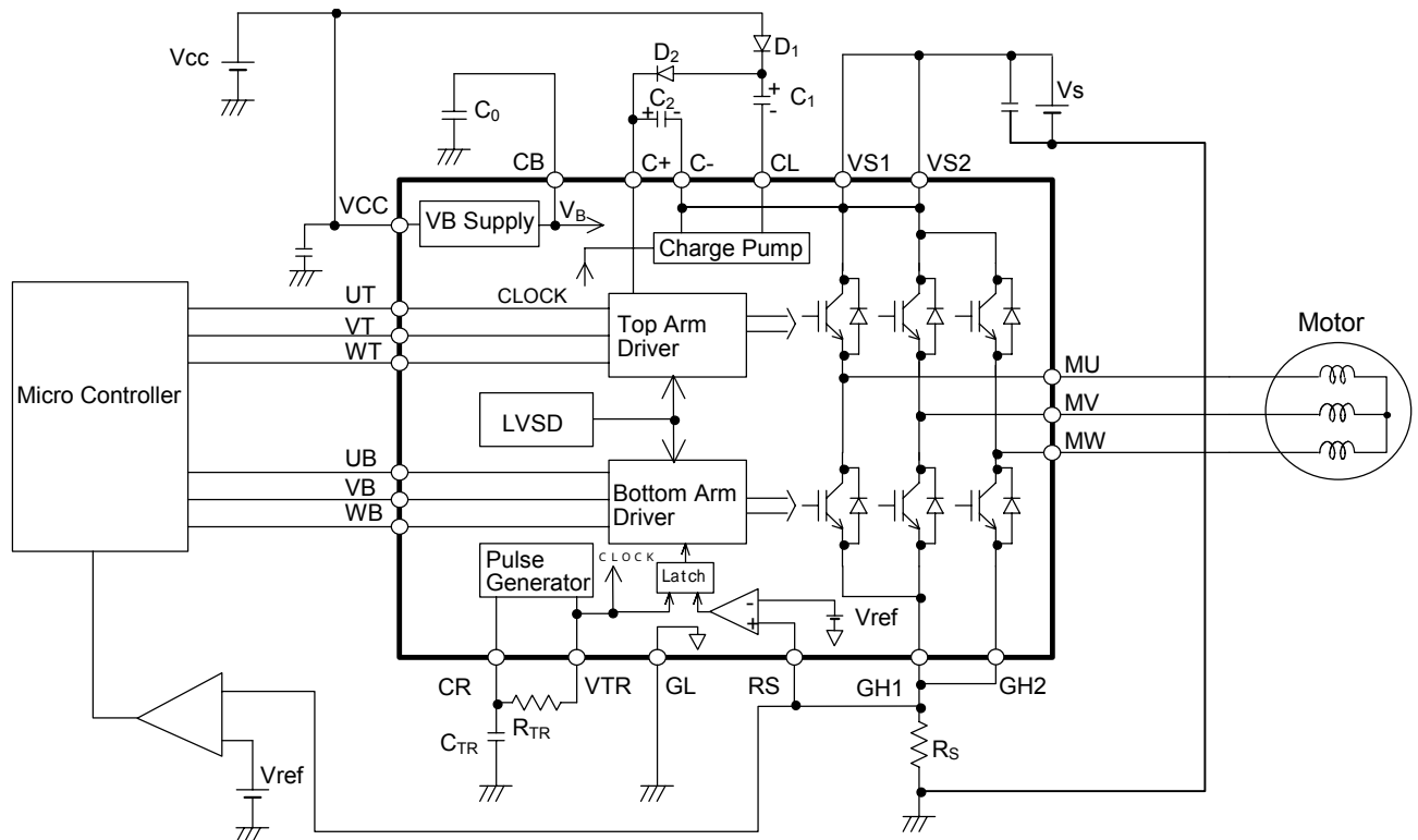
Figure 4. Block Diagram
